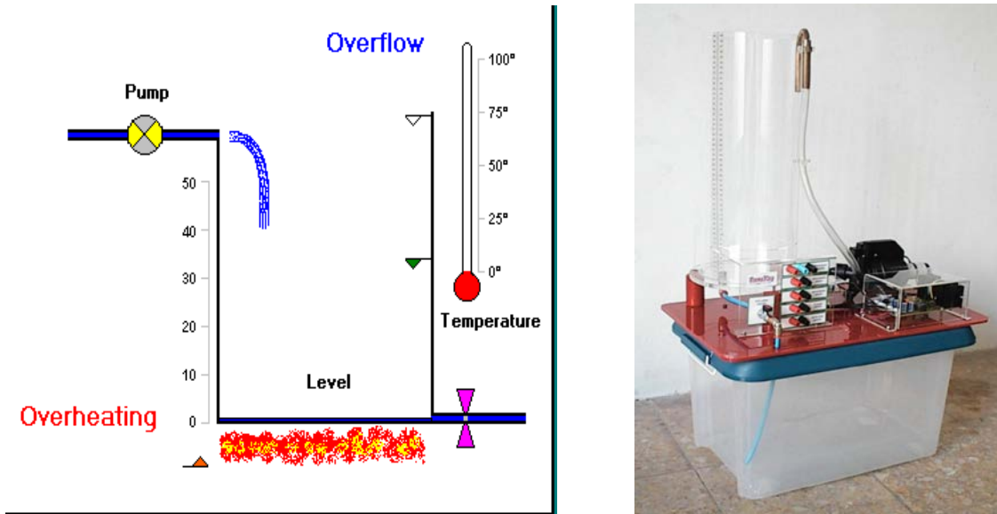
Figure 2.1-2 Liquids tank process
